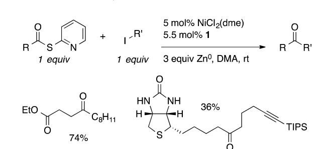
Scheme 5. Nickel-Catalyzed Coupling of 2-Pyridyl Thioesters with Alkyl Iodides
