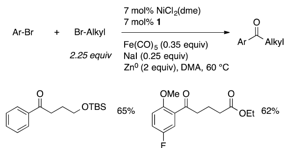
Scheme 9. Carbonylative Cross-Coupling
