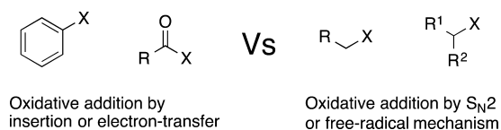
Figure 3. Generally selective cross-electrophile reactions were envisioned to be possible between Csp^2-X and Csp^3-X bonds because the mechanisms of oxidative addition are different.
